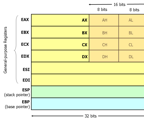
Figure 1. x86 Registers
